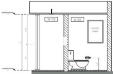
ELEVATION B2 0 - 1/2" = 1'-0"
